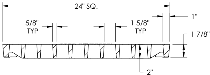
SECTION B-B
